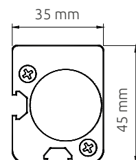
Cross section
