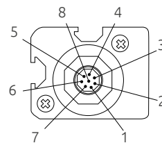
Receiver M12 8-pole
